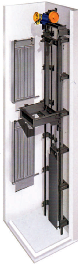
MRL structure dimensions
